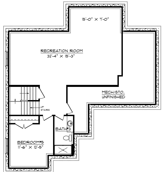
Finished Basement
